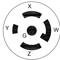
L21-30P PLUG END
